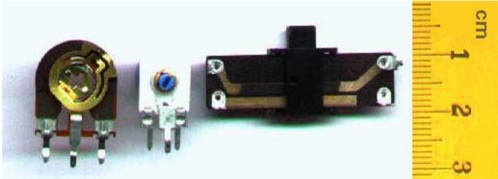
Abb. 6: Potentiometer
